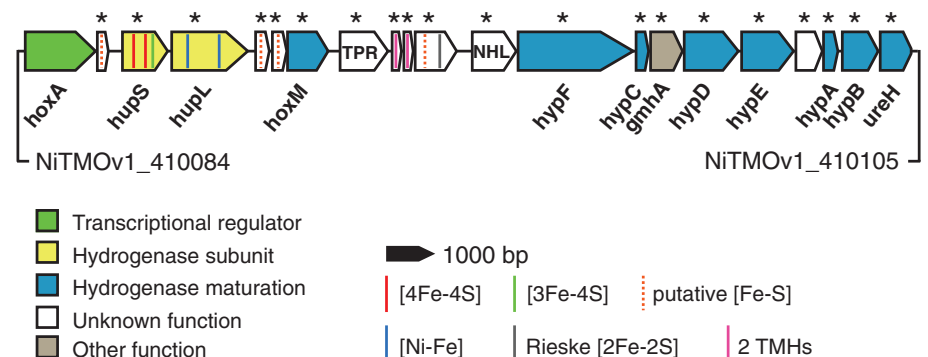
Fig. 1. Schematic illustration of the hydrogenase ( hup ) locus of N. moscoviensis . Predicted structural features or domains are marked with colored vertical lines. TPR (tetratricopeptide repeats), or NHL (NHL repeats). Asterisks indicate significant gene up-regulation (DESeq P_{adj} < 0.05 , fold change \geq 2 ) under H 2 -oxidizing conditions, as detected by whole transcriptome shotgun sequencing. Genes are drawn to scale. TMH, transmembrane helix.
